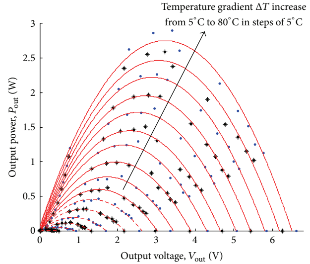
FIGURE 12: The output power, P_{out} [W], versus the output voltage, V_{out} [V], for different temperature gradient, \Delta T [°C].
